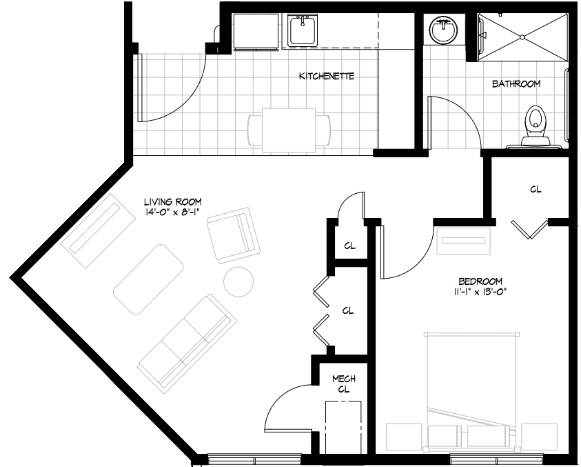
ONE BEDROOM/ONE BATHROOM
